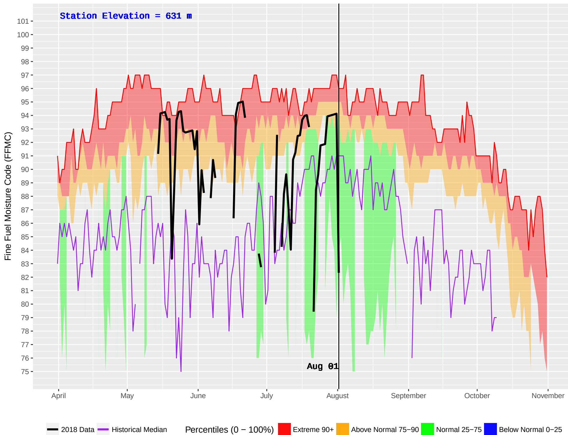
EAST BARRIERE (243) : Historical (1978–2016) and Current (2018) Daily Fine Fuel Moisture Code (FFMC)
