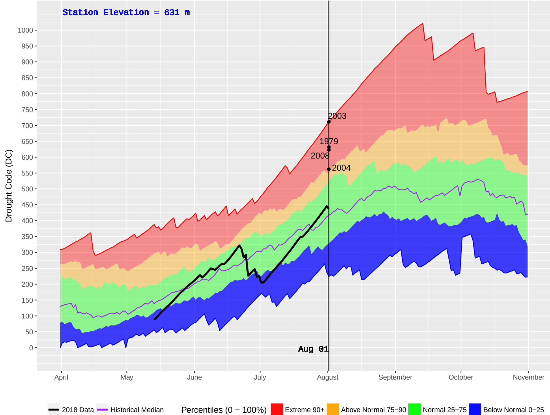
EAST BARRIERE (243) : Historical (1978–2016) and Current (2018) Daily Drought Code (DC)
