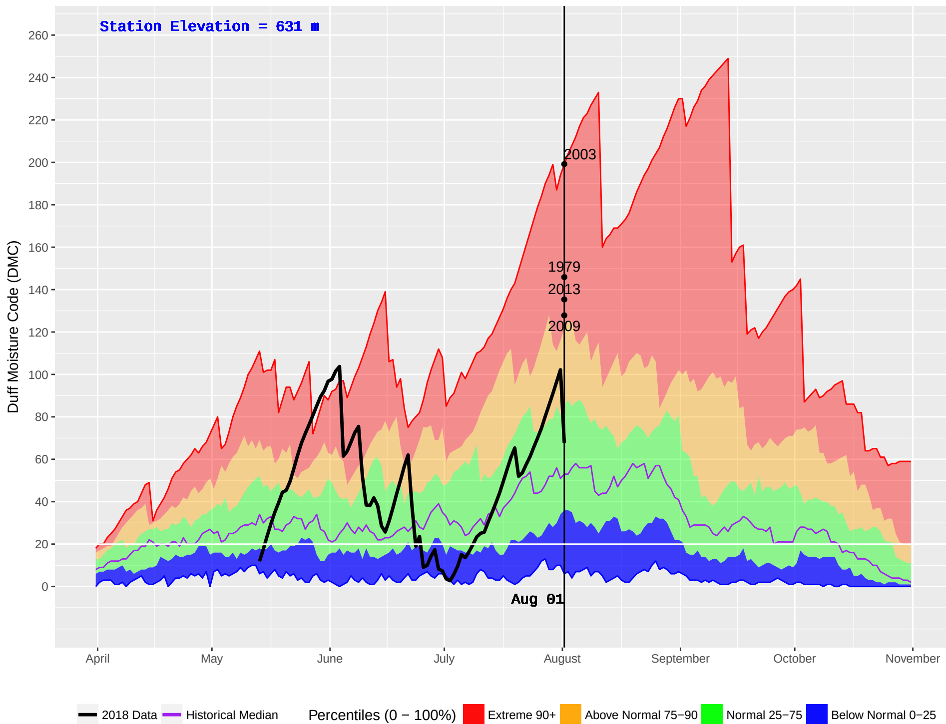
EAST BARRIERE (243) : Historical (1978–2016) and Current (2018) Daily Duff Moisture Code (DMC)
