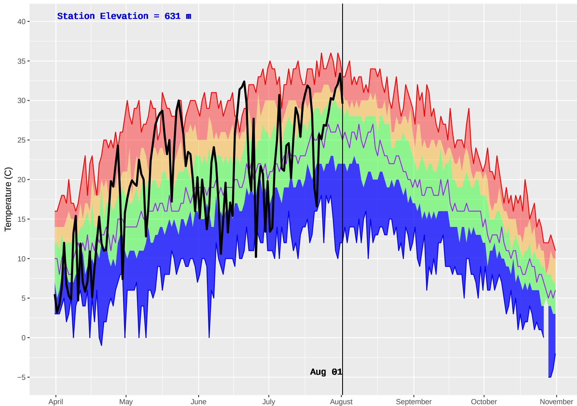
EAST BARRIERE (243) : Historical (1978–2016) and Current (2018) Daily Temperature
