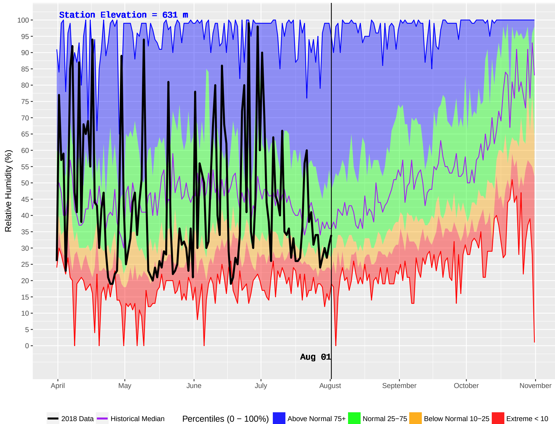
EAST BARRIERE (243) : Historical (1978–2016) and Current (2018) Daily Relative Humidity
