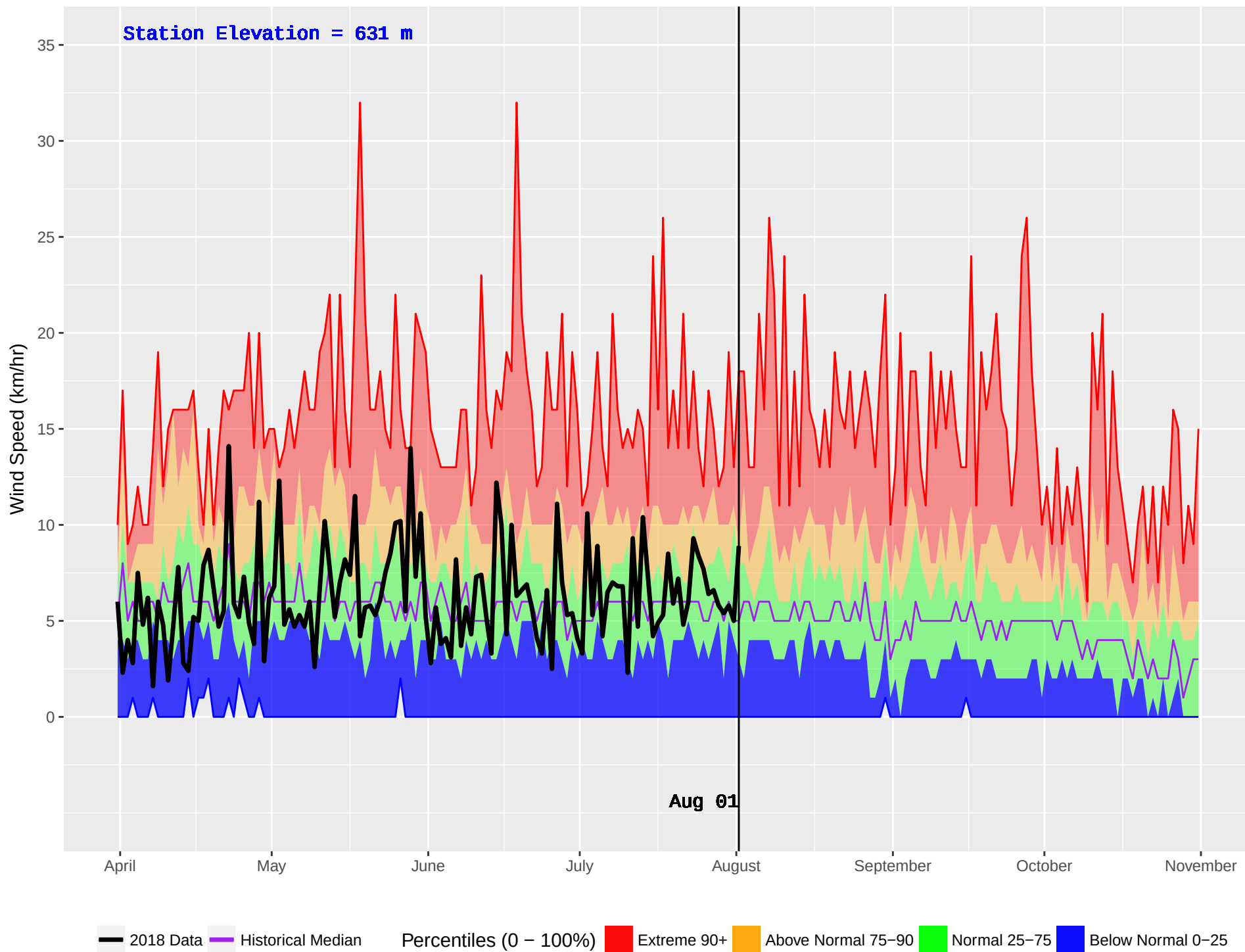
EAST BARRIERE (243) : Historical (1978–2016) and Current (2018) Daily Wind Speed
