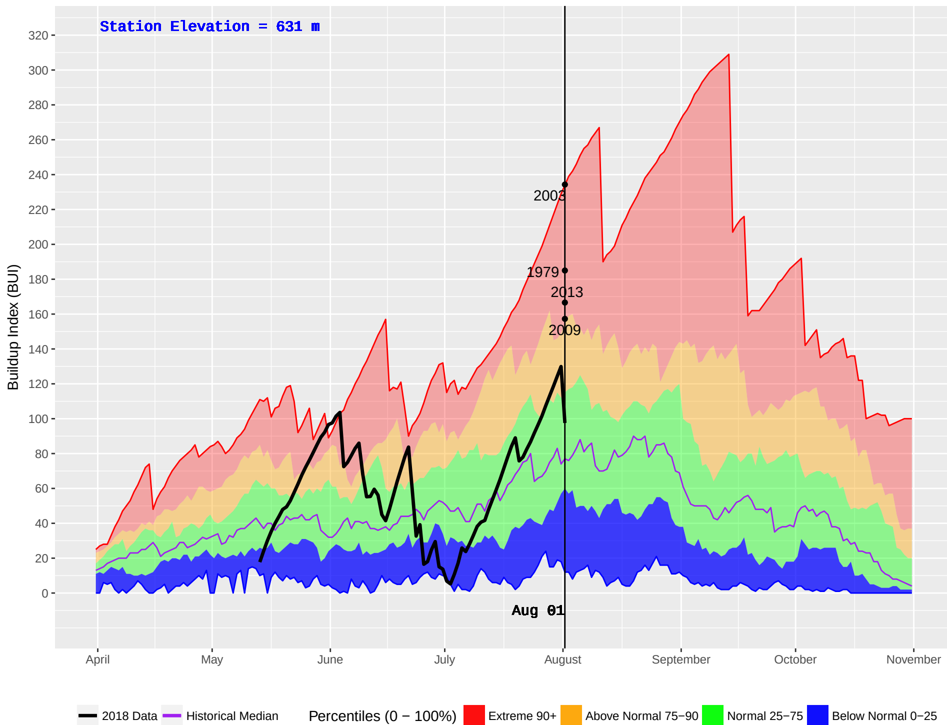
EAST BARRIERE (243) : Historical (1978–2016) and Current (2018) Daily Buildup Index (BUI)
