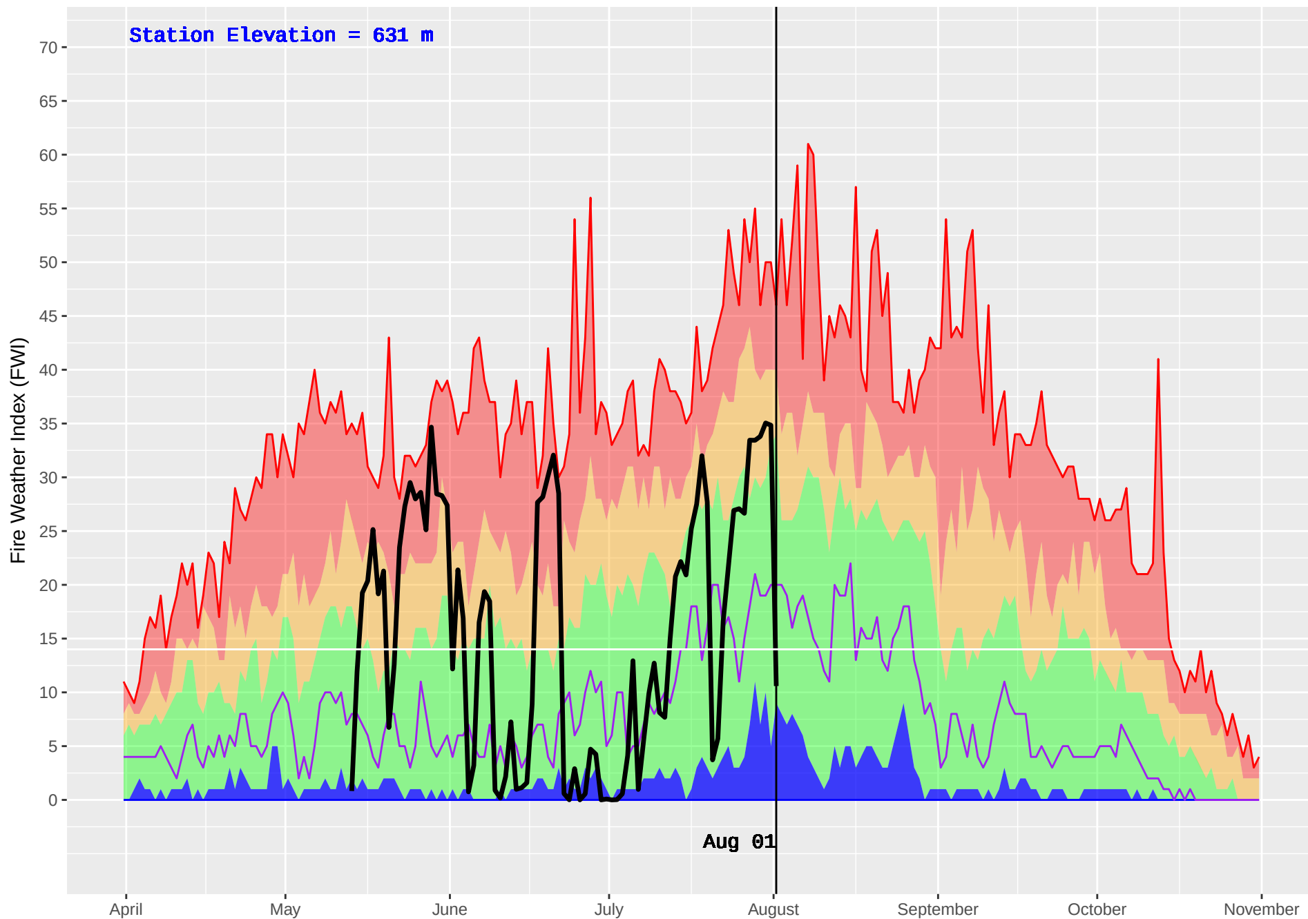
EAST BARRIERE (243) : Historical (1978–2016) and Current (2018) Daily Fire Weather Index (FWI)
